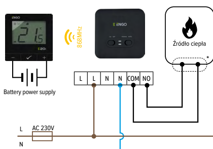
a) Connection diagrams to the heat source
