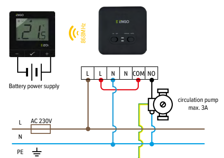
c) Connection diagrams for the circulation pump
