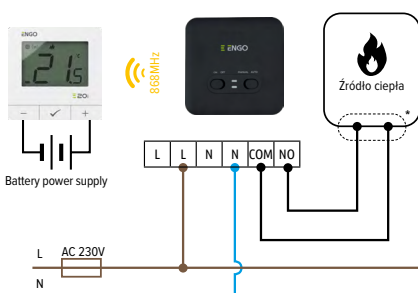
a) Connection diagrams to the heat source
