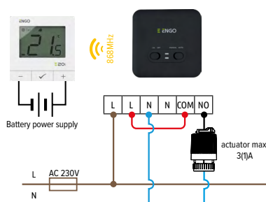
b) Connection diagrams for the actuator
