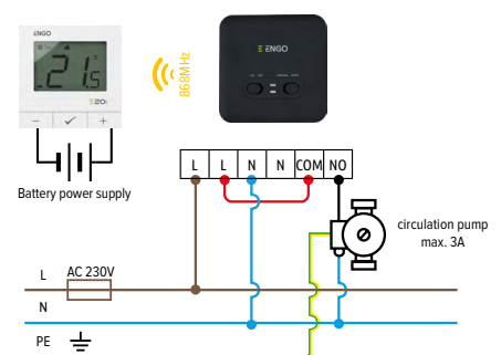
c) Connection diagrams for the circulation pump
